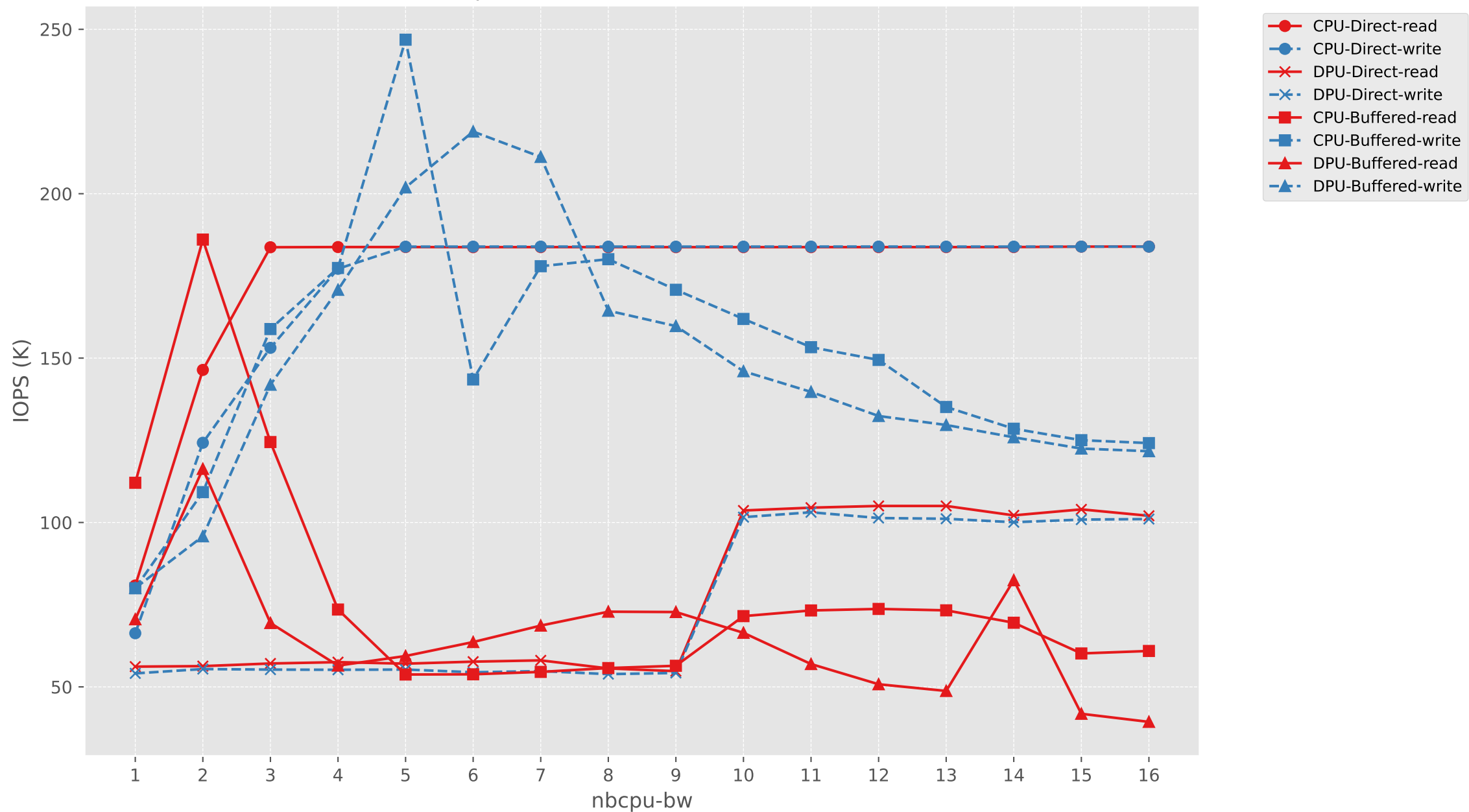
IOPS vs nbcpu-bw (CPU vs DPU, Direct vs Buffered)
